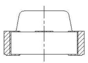
剖面图 Section View
