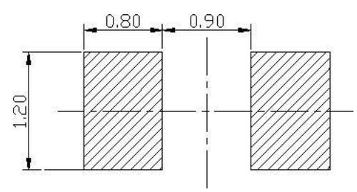
推荐焊盘尺寸 Recommended Soldering Pad
