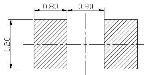
推荐焊盘尺寸 Recommended Soldering Pad
