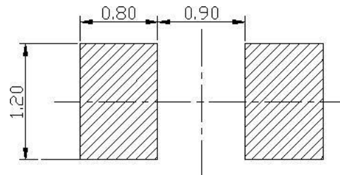
推荐焊盘尺寸 Recommended Soldering Pad
